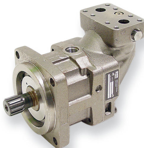
▲ VOAC Hydrostatic Motor - Fan Vacuum Systems 622-0219
