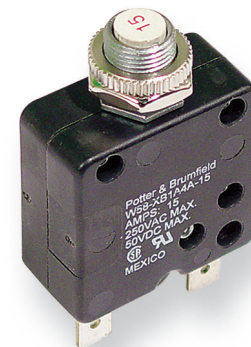
▲ Circuit Breaker Part Number Description 630-0081 5 AMP 630-0082 10 AMP 630-0083 15 AMP 630-0176 20 AMP 630-0198 25 AMP
