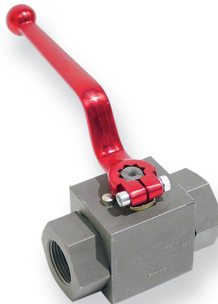
▲ Hycon 1" 2 Way Ball Valve 662-0205 — 3000PSI
