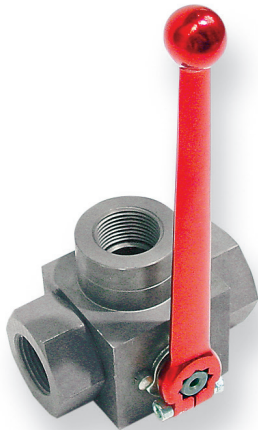
▲ Hycon 1" 3 Way Ball Valve 662-0003 — 2500 PSI
